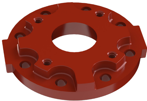
3" ANSI side featuring threaded 3" ANSI pattern and clearance for 5/8" - 11 screw hex heads
